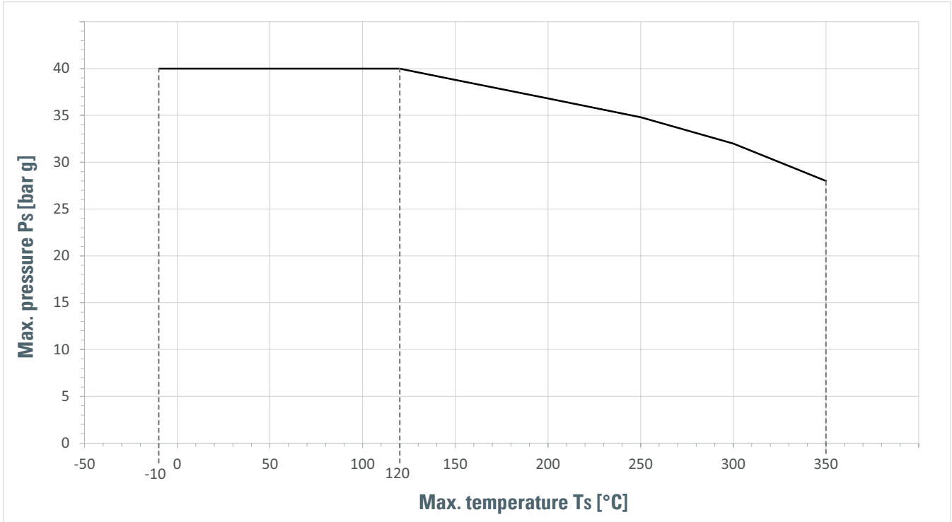
Pressure-temperature relationship above 50°C according to DIN EN 1092-2.
