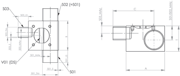
T valve
