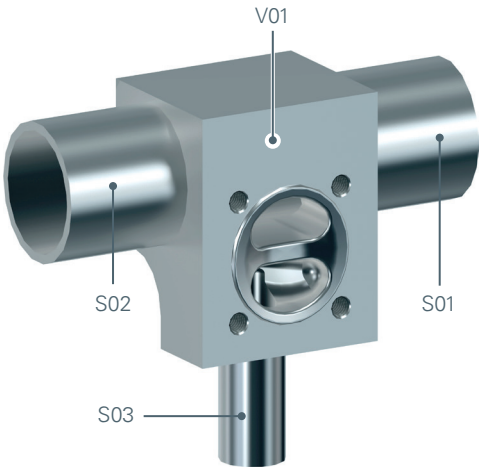
Body design 0301TNL
